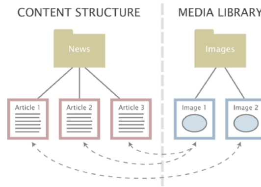
Figure 1.16: Object relations.
