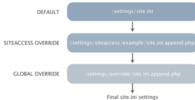
Figure 2.23: Configuration override example.
