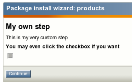
Figure 4.64: Displaying a custom wizard step during the package installation process
