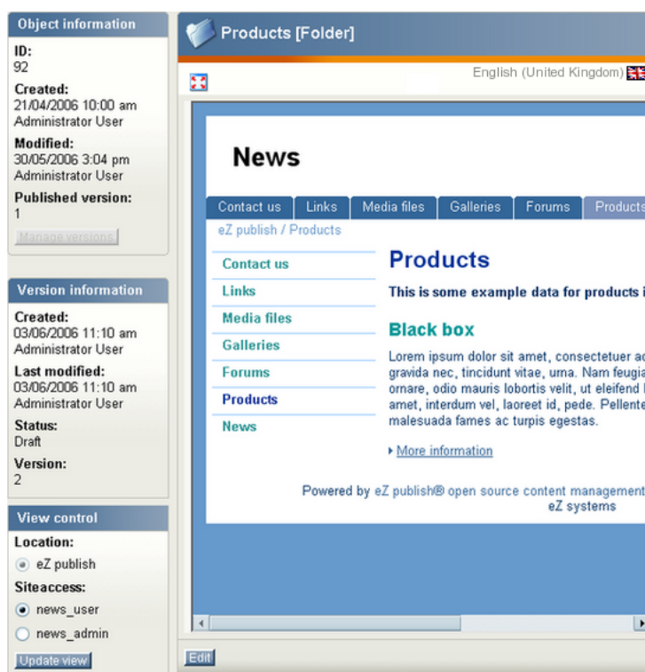
Figure 1.24: The preview interface.
