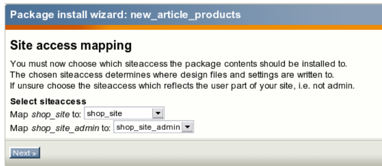
Figure 4.41: The content object package installation wizard, step 2.
